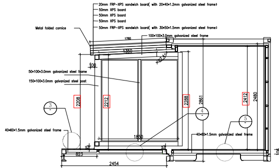
Cross Section B-D Side Headroom SCALE 1:30
