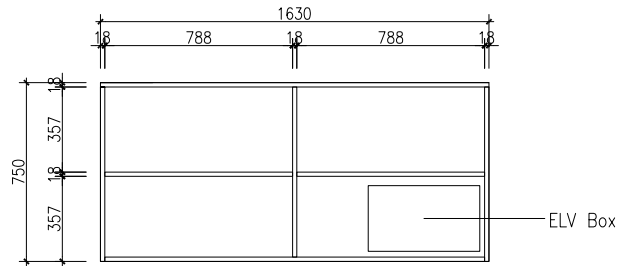
Overhead Cupboards Inner Layout
