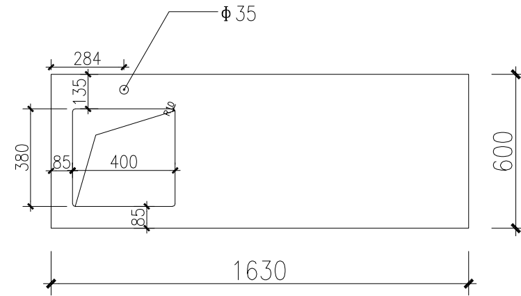
Kitchen Bench Openings on quartz countertop SCALE 1:30
