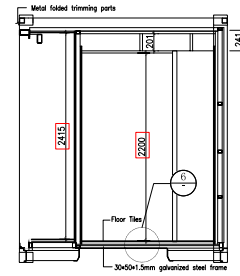
Cross Section B-D Side Bathroom Headroom SCALE 1:30
