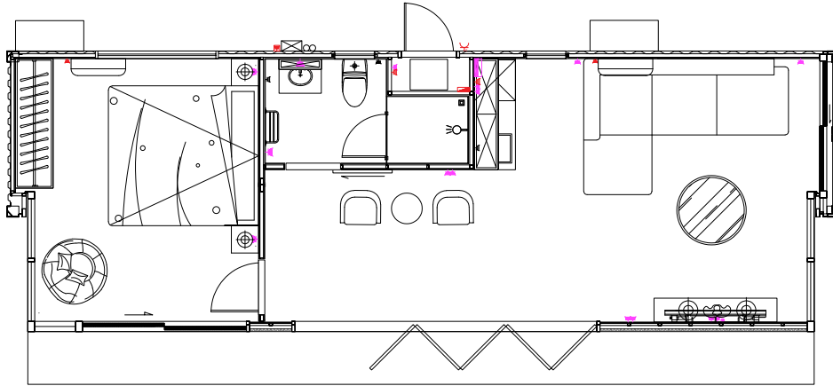
Electrical Plan Power Points SCALE 1:30
