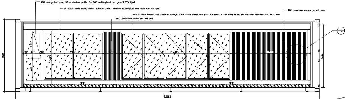
EXTERIOR ELEVATION A Side (Open State) SCALE 1:30
