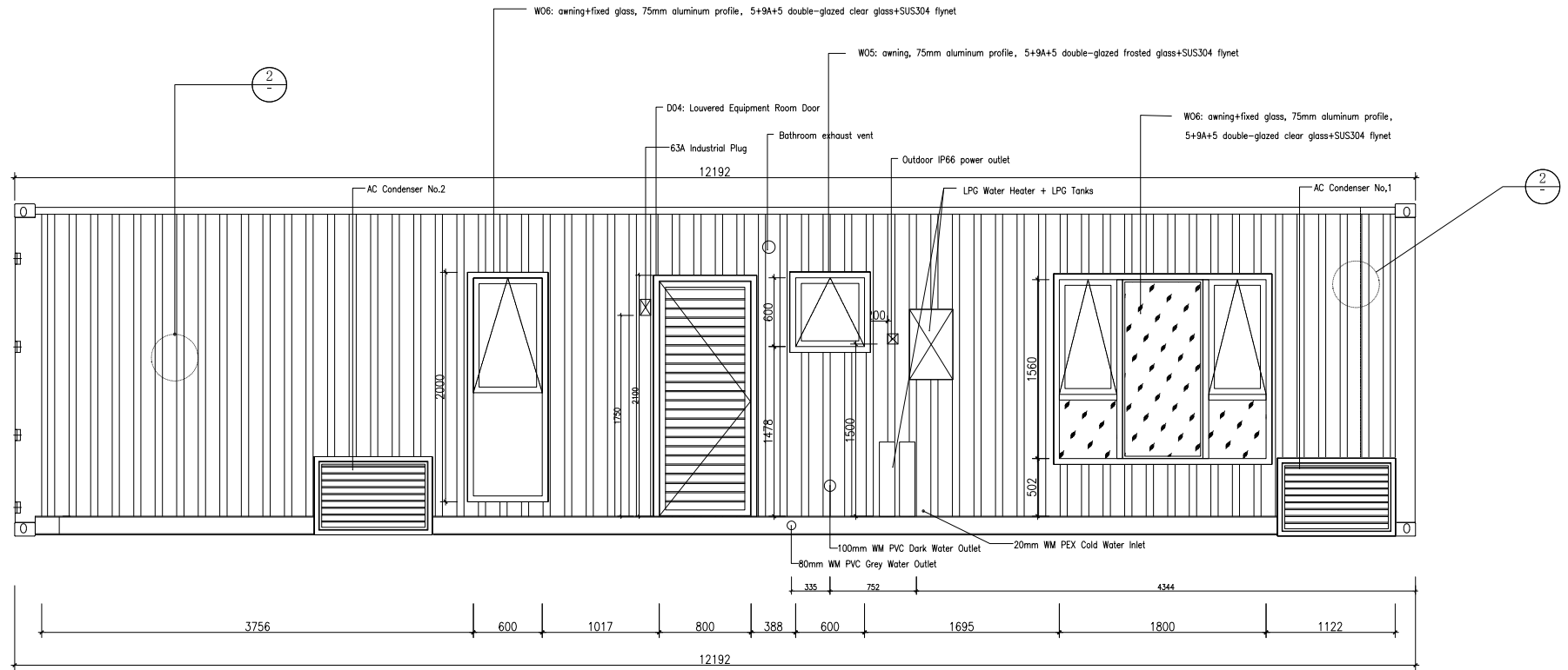
EXTERIOR ELEVATION C Side SCALE 1:30
