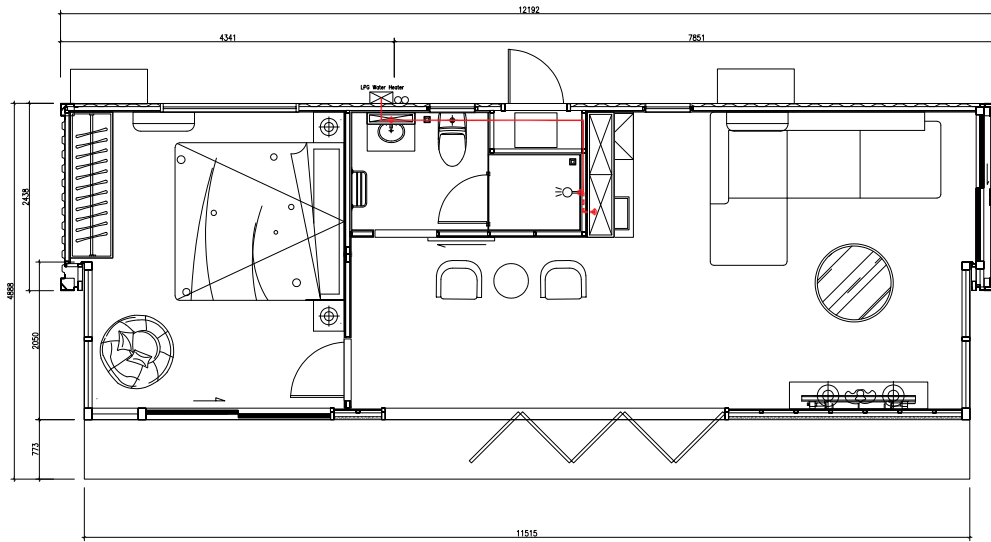
PLUMBING PLAN Hot Water Supply SCALE 1:30
