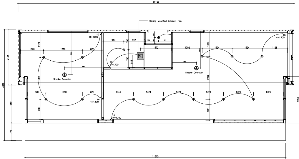
Electrical Plan RCP SCALE 1:30
