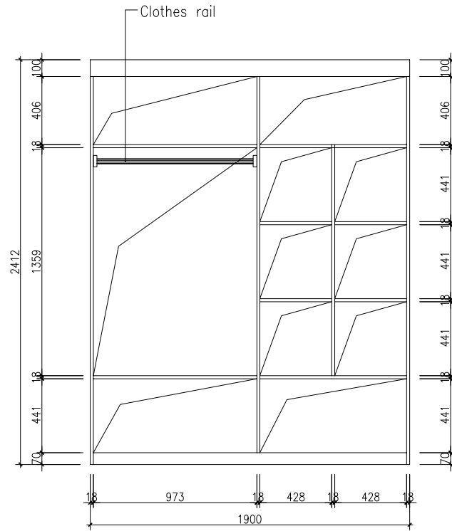
Inner Layout SCALE 1:30
