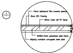
Cross Section B-D Side Headroom SCALE 1:30
