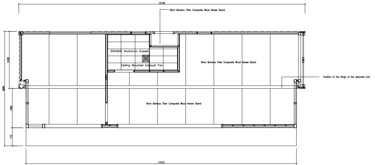
LAYOUT PLAN Ceiling SCALE 1:30
