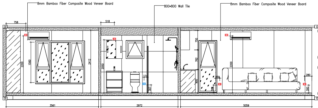
INTERIOR ELEVATION Power Points Location (C Side) SCALE 1:30
