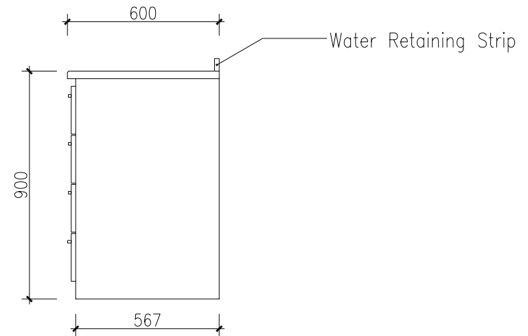
Kitchen Bench Side View
