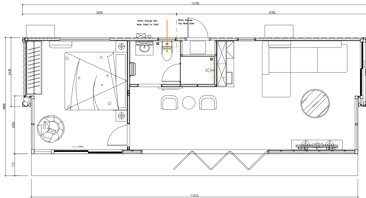
PLUMBING PLAN West Water Line SCALE 1:30
