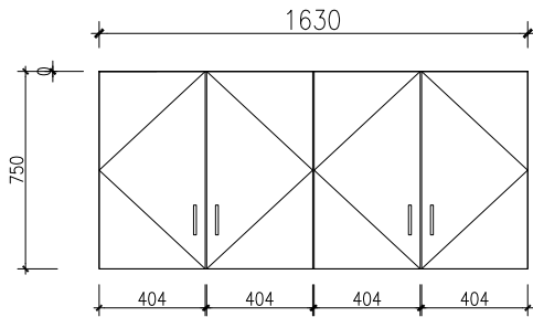
Overhead Cupboards Front View
