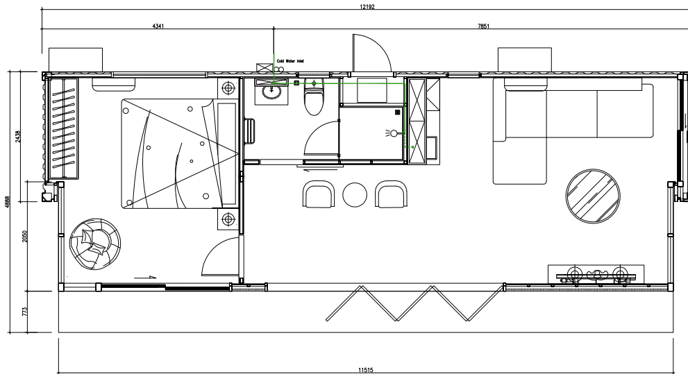
PLUMBING PLAN Cold Water Supply SCALE 1:30
