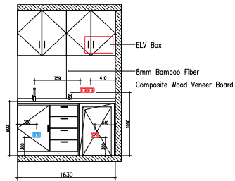
INTERIOR ELEVATION Power Points Location (Kitchen Backwall) SCALE 1:30
