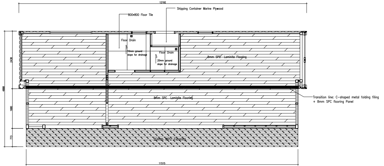
LAYOUT PLAN Flooring SCALE 1:30
