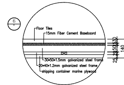
Cross Section B-D Side Bathroom Headroom SCALE 1:30
