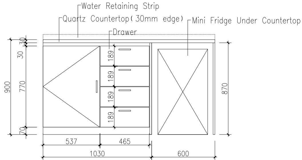
Kitchen Bench Front View
